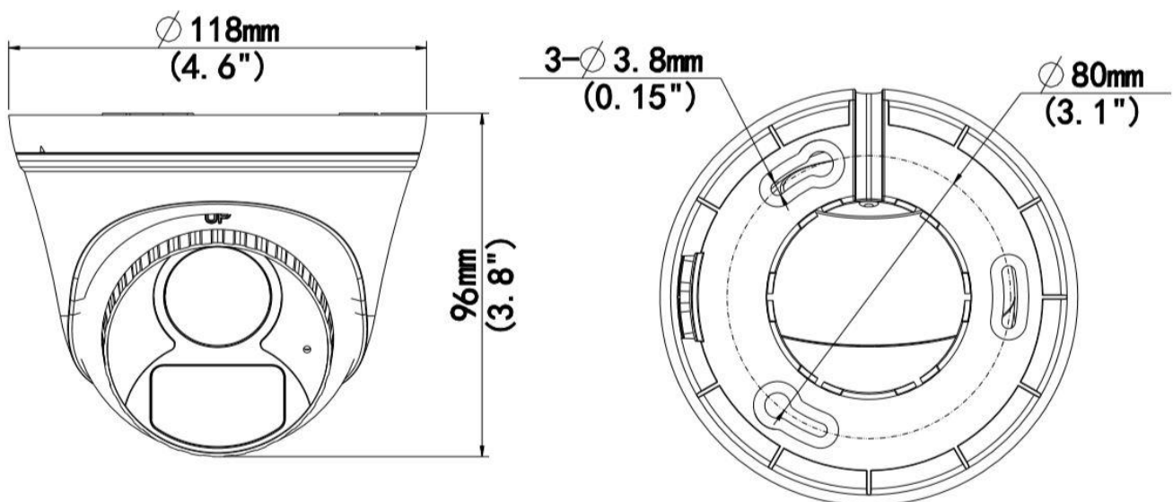
UAC-T112-AF28(40)-W
